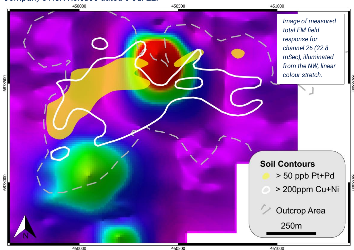
Figure 2: Waratah Well – Ni-Cu-PGE Drill Target
