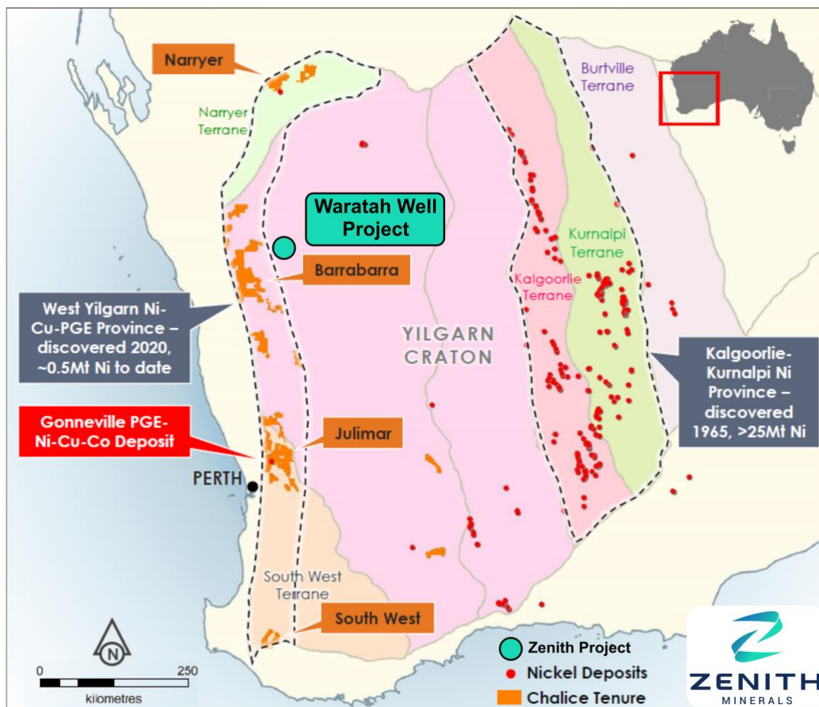
Figure 1: Waratah Well Project Area with Respect to the West Yilgarn Ni-Cu-PGE Province
